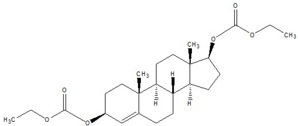
4-Androstene-3,17-diethylcarbonate ester
